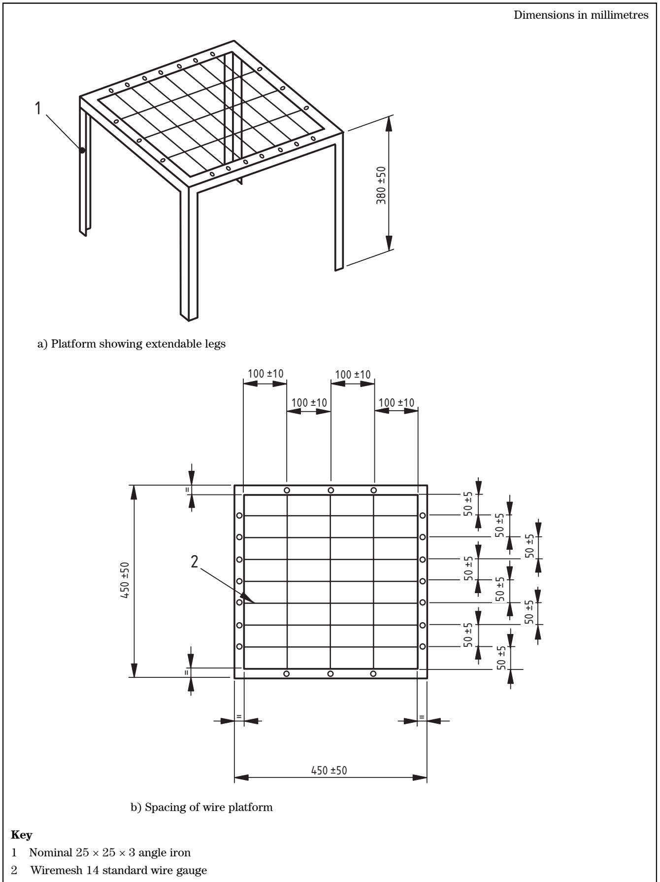
Figure 2 Test rig
