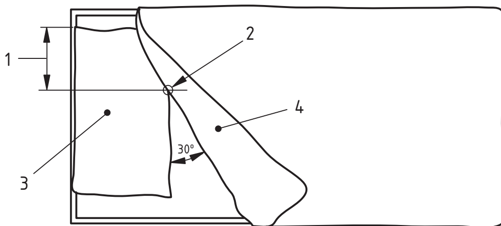
Figure 4 Position of ignition sources for mattresses tested with secondary ignition sources of known bed covers
